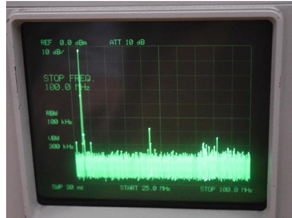
Tuner matched (52dBc)
