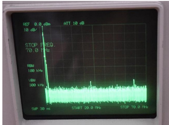
Tuner matched (65dBc)
