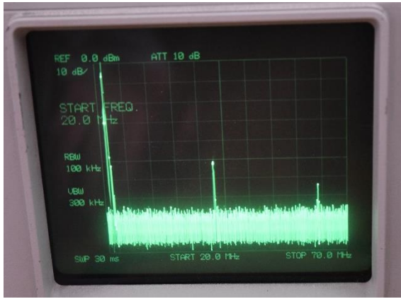
21225KHz Tuner through (50dBc)
