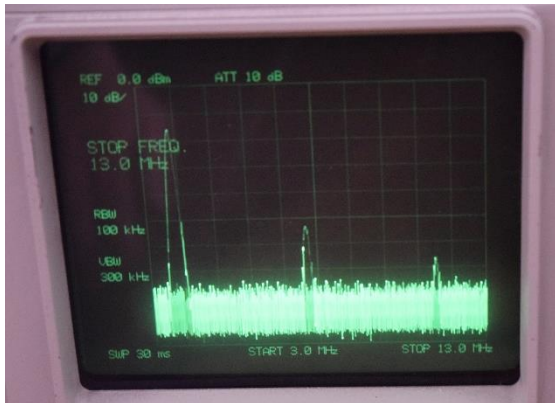
3793KHz Tuner through (35dBc)
